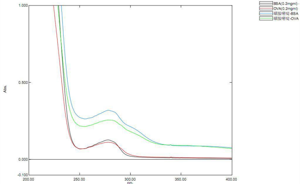
Figure 2. UV-spectrum
