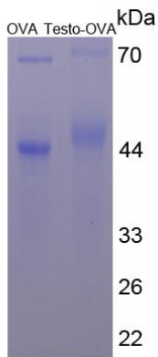
Figure 1. SDS-PAGE
