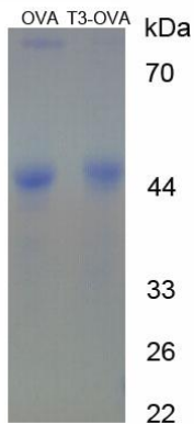
Figure 1. SDS-PAGE
