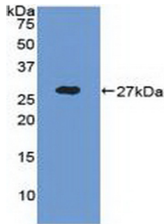
Figure. Western Blot; Sample: Recombinant ADAM17, Human.
