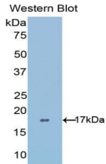
Figure. Western Blot; Sample: Recombinant ADAMTS4, Human.
