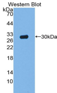
Figure. Western Blot; Sample: Recombinant ACP5, Mouse.
