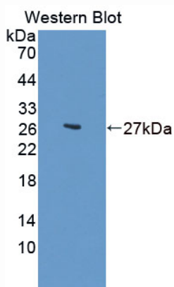
Used in Western Blot, Sample: Recombinant ATR, Human
