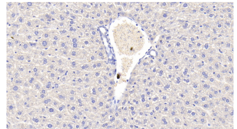
DAB staining on IHC-P; Samples: Mouse Liver Tissue; Primary Ab: 20µg/ml Rabbit Anti-Mouse CRP Antibody Second Ab: 2µg/mL HRP-Linked Caprine Anti-Rabbit IgG Polyclonal Antibody (Catalog: SAA544Rb19)
