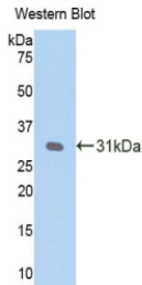
Figure. Western Blot; Sample: Recombinant CRP, Mouse.
