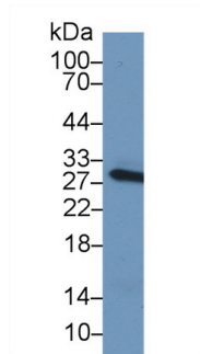
Western Blot; Sample: Mouse Serum; Primary Ab: 1µg/ml Rabbit Anti-Mouse CRP Antibody Second Ab: 0.2µg/mL HRP-Linked Caprine Anti-Rabbit IgG Polyclonal Antibody (Catalog: SAA544Rb19)
