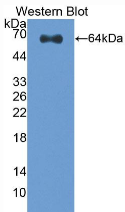
Used in Western Blot, Sample: Recombinant CLEC11A, Human
