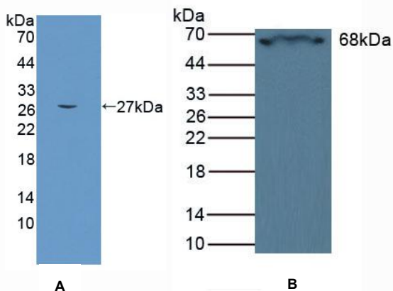
Figure 1. Western Blot
