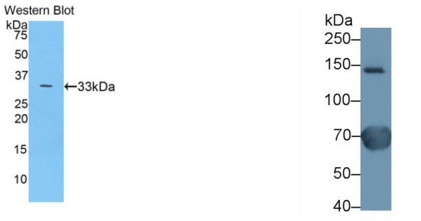
Figure. Western Blot; Sample: Recombinant Ceruloplasmin, Human. Western Blot; Sample: Rat Serum; Primary Ab: 1µg/ml Rabbit Anti-Human CP Antibody Second Ab: 0.2µg/mL HRP-Linked Caprine Anti-Rabbit IgG Polyclonal Antibody (Catalog: SAA544Rb19)
