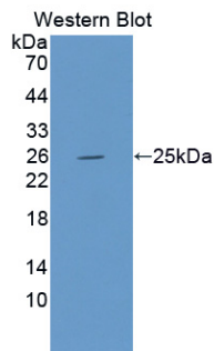
Figure. Western Blot; Sample: Recombinant CHD5, Human.
