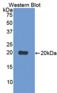
Figure. Western Blot; Sample: Recombinant CD30L, Human.
