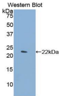
Figure. Western Blot; Sample: Recombinant CLEC4M, Human.
