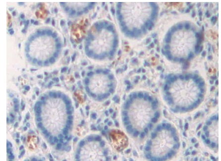
DAB staining on IHC-P; Samples: Human Stomach Tissue; Primary Ab: 10µg/ml Rabbit Anti-Human CLEC4M Antibody Second Ab: 2µg/mL HRP-Linked Caprine Anti-Rabbit IgG Polyclonal Antibody (Catalog: SAA544Rb19)
