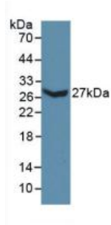
Figure. Western Blot; Sample: Recombinant COL3a1, Mouse.
