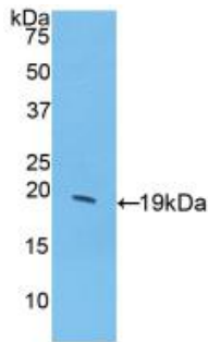
Figure. Western Blot; Sample: Recombinant GCSF, Porcine.
