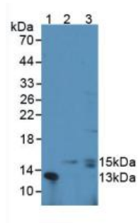
Figure. Western Blot; Sample: Lane1: Mouse Lymphocyte Cells; Lane2: Human Leukocyte Cells; Lane3: Mouse Thymus Tissue.
