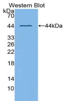
Figure. Western Blot; Sample: Recombinant CDK2, Human.
