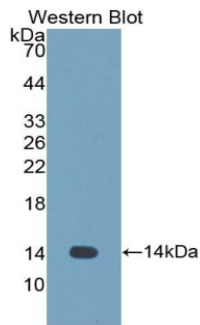
Figure. Western Blot; Sample: Recombinant CST1, Human.
