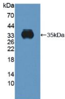
Figure. Western Blot; Sample: Recombinant CYBb, Human.
