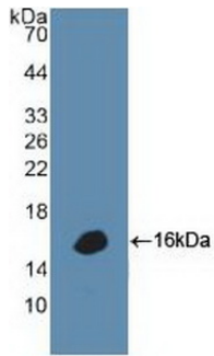
Figure. Western Blot; Sample: Recombinant DEFa1, Human.
