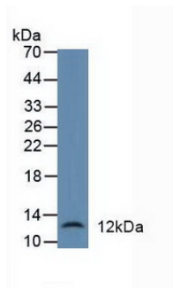
Figure. Western Blot; Sample: Human Liver Tissue.
