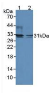
Figure. Western Blot; Sample: Lane1: Rat Brain Tissue; Lane2: Mouse Brain Tissue.
