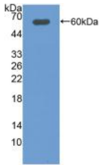
Figure. Western Blot; Sample: Recombinant DIO2, Rat.
