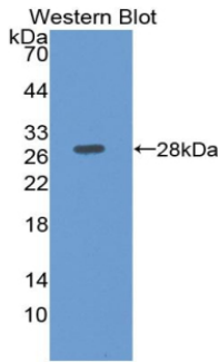
Figure. Western Blot; Sample: Recombinant dLK1, Rat.
