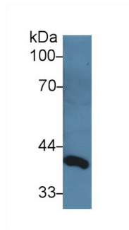
Western Blot; Sample: Rat Serum; Primary Ab: 3µg/ml Rabbit Anti-Rat dLK1 Antibody Second Ab: 0.2µg/mL HRP-Linked Caprine Anti-Rabbit IgG Polyclonal Antibody (Catalog: SAA544Rb19)
