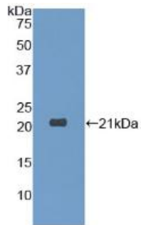
Figure. Western Blot; Sample: Recombinant DPT, Human.
