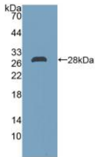
Figure. Western Blot; Sample: Recombinant DDAH2, Human.
