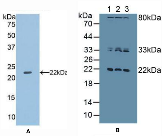
Figure 1. Western Blot
