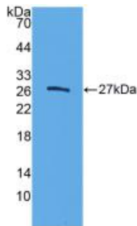
Figure. Western Blot; Sample: Recombinant ELA3B, Human.
