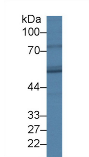
Western Blot; Sample: Porcine Stomach lysate; Primary Ab: 2µg/ml Rabbit Anti-Human FADS3 Antibody Second Ab: 0.2µg/mL HRP-Linked Caprine Anti-Rabbit IgG Polyclonal Antibody (Catalog: SAA544Rb19)
