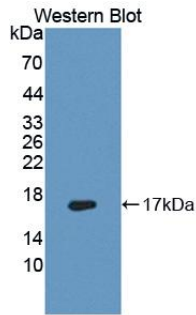
Figure. Western Blot; Sample: Recombinant FADS3, Human.
