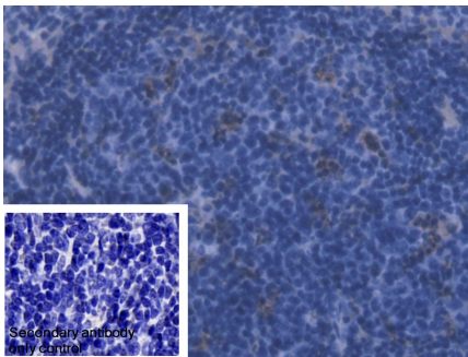
DAB staining on IHC-P; Sample: Mouse Spleen Tissue
