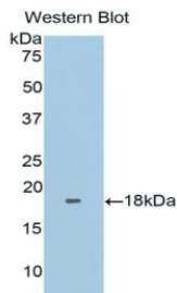
Figure. Western Blot; Sample: Recombinant FNDC5, Human.
