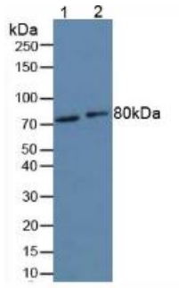
Figure. Western Blot; Sample. Lane1: Human Hela Cells; Lane2: Mouse Liver Tissue.
