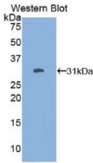
Figure. Western Blot; Sample: Recombinant FOXO1, Rat.
