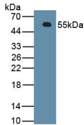
Figure. Western Blot; Sample: Recombinant FXR, Rat.
