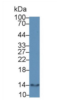
Western Blot; Sample: Porcine Skeletal muscle lysate; Primary Ab: 5µg/ml Rabbit Anti-Bovine GAL1 Antibody Second Ab: 0.2µg/mL HRP-Linked Caprine Anti-Rabbit IgG Polyclonal Antibody (Catalog: SAA544Rb19)
