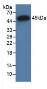
Figure. Western Blot; Sample: Recombinant GR, Human.
