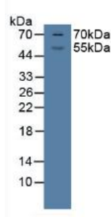
Figure. Western Blot; Sample: Porcine Brian Tissue.
