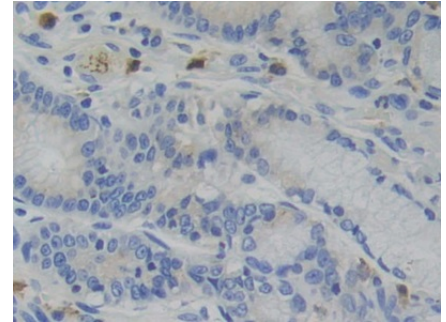
DAB staining on IHC-P; Samples: Human Stomach Tissue; Primary Ab: 10µg/ml Rabbit Anti-Human NR3C1 Antibody Second Ab: 2µg/mL HRP-Linked Caprine Anti-Rabbit IgG Polyclonal Antibody (Catalog: SAA544Rb19)
