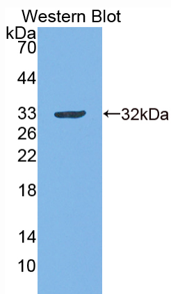
Used in Western Blot, Sample: Recombinant GBP6, Human
