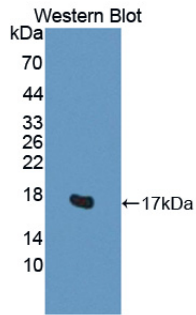
Figure. Western Blot; Sample: Recombinant H2AFV, Human.
