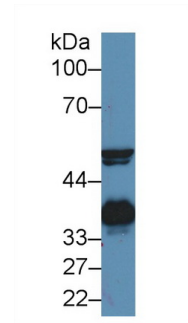
Western Blot; Sample: Bovine Serum; Primary Ab: 5µg/ml Rabbit Anti-Bovine Hpt Antibody Second Ab: 0.2µg/mL HRP-Linked Caprine Anti-Rabbit IgG Polyclonal Antibody (Catalog: SAA544Rb19)
