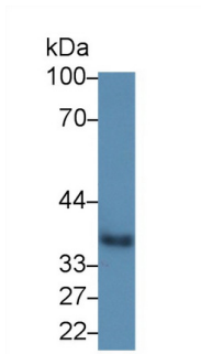
Western Blot; Sample: Bovine Liver lysate; Primary Ab: 5µg/ml Rabbit Anti-Bovine Hpt Antibody Second Ab: 0.2µg/mL HRP-Linked Caprine Anti-Rabbit IgG Polyclonal Antibody (Catalog: SAA544Rb19)
