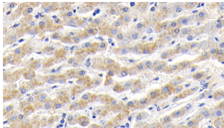
DAB staining on IHC-P; Samples: Bovine Liver Tissue; Primary Ab: 20?g/ml Rabbit Anti-Bovine Hpt Antibody Second Ab: 2µg/mL HRP-Linked Caprine Anti-Rabbit IgG Polyclonal Antibody (Catalog: SAA544Rb19)
