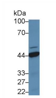
Western Blot; Sample: Human Hela cell lysate; Primary Ab: 5µg/ml Rabbit Anti-Bovine Hpt Antibody Second Ab: 0.2µg/mL HRP-Linked Caprine Anti-Rabbit IgG Polyclonal Antibody (Catalog: SAA544Rb19)
