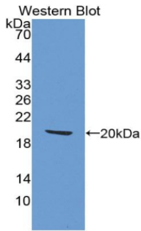
Figure. Western Blot; Sample: Recombinant HBEGF, Mouse.
