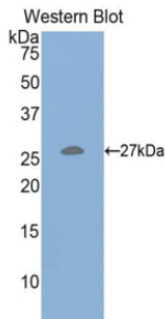
Figure. Western Blot; Sample: Recombinant HGF, Mouse.
