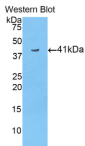
Figure. Western Blot; Sample: Recombinant HIST3H2A, Human.
