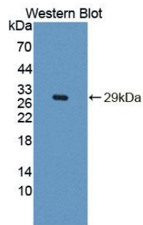
Figure. Western Blot; Sample: Recombinant IRS4, Human.
