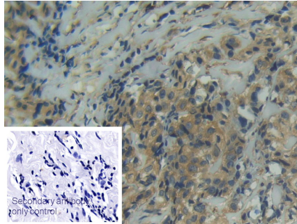
DAB staining on IHC-P; Sample: Human Breast cancer Tissue; Primary Ab: 20µg/ml Rabbit Anti-Human ITGaD Antibody Second Ab: 2µg/mL HRP-Linked Caprine Anti-Rabbit IgG Polyclonal Antibody (Catalog: SAA544Rb19) Secondary antibody only control: Used PBS instead of primary antibody, Second Ab: 2µg/mL HRP
