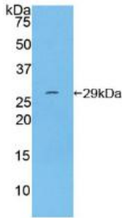
Figure. Western Blot; Sample: Recombinant ITGaD, Human.
