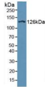
Figure. Western Blot; Sample: Human Serum.
