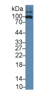
Western Blot; Sample: Human HL60 cell lysate; Primary Ab: 1µg/ml Rabbit Anti-Human ICAM3 Antibody Second Ab: 0.2µg/mL HRP-Linked Caprine Anti-Rabbit IgG Polyclonal Antibody (Catalog: SAA544Rb19)
