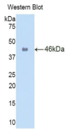
Figure. Western Blot; Sample: Recombinant IL1b, Mouse.
