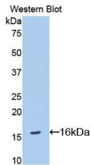
Figure. Western Blot; Sample: Recombinant IL18R1, Mouse.
