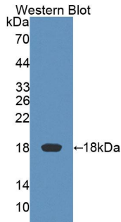
Figure. Western Blot; Sample: Recombinant KLRK1, Rat.
