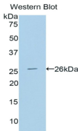
Figure. Western Blot; Sample: Recombinant Laminin, Rat.
