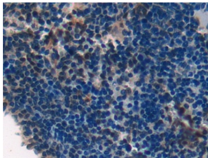
DAB staining on IHC-P; Samples: Mouse Spleen Tissue; Primary Ab: 10µg/ml Rabbit Anti-Mouse LAMa1 Antibody Second Ab: 2µg/mL HRP-Linked Caprine Anti-Rabbit IgG Polyclonal Antibody (Catalog: SAA544Rb19)
