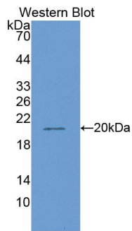
Figure. Western Blot; Sample: Recombinant MMP13, Rabbit.
