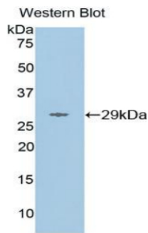
Figure. Western Blot; Sample: Recombinant MMP16, Human.
