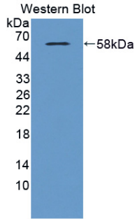
Figure. Western Blot; Sample: Recombinant GRM3, Human.
